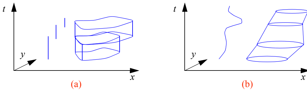
Figure 1.11: (a) Discretely changing point and region (b) Continuously changing point and region
